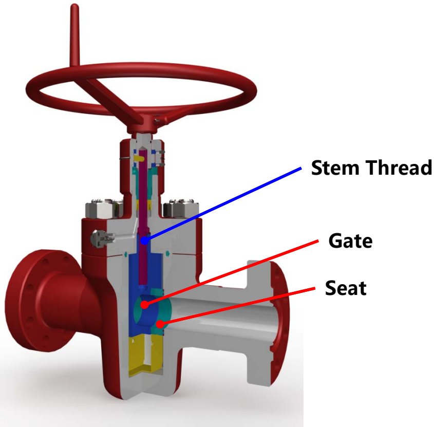
Neway GBS Slab Gate Valve
